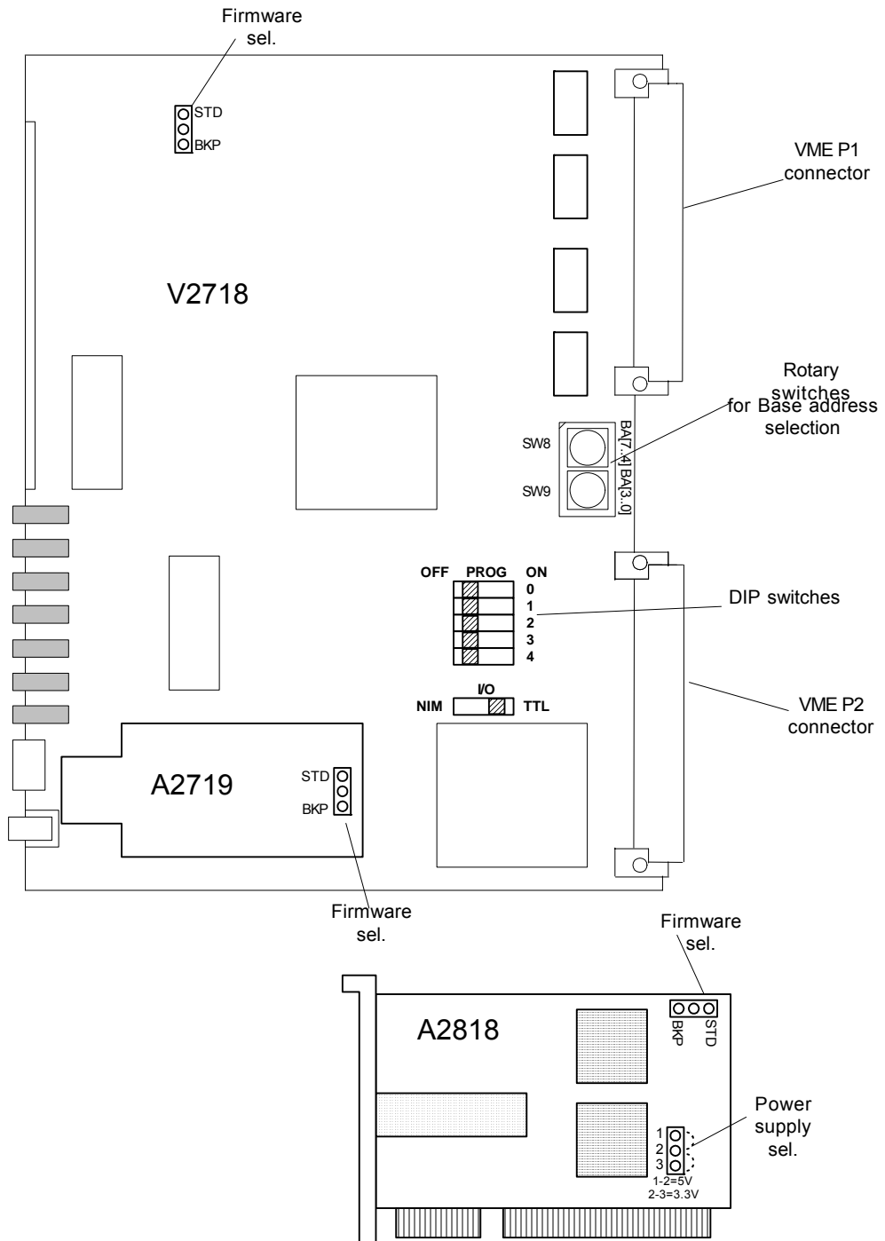
Fig. 3.3: Component Location
