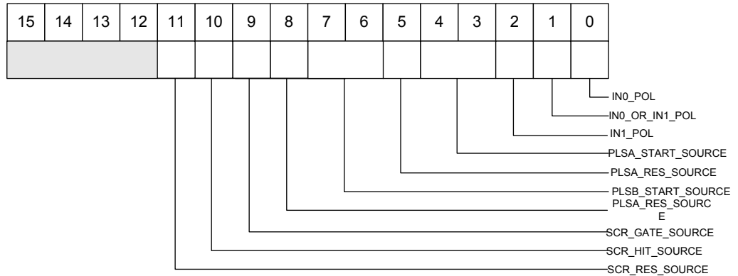
Fig. 2.13: Input Multiplexer register
